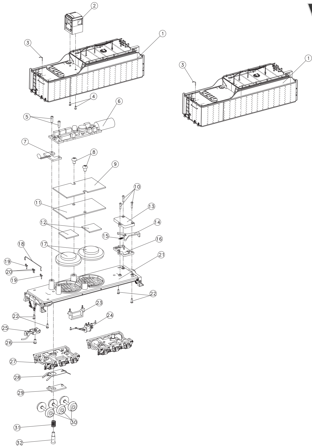
Texas & Pacific 2-10-4 Tender Exploded View Diagram
