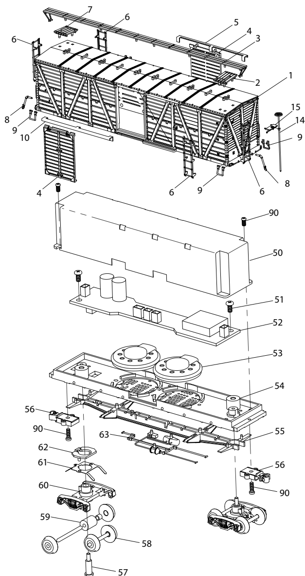
K7 Stock Car (With Sound) Exploded View Diagram
