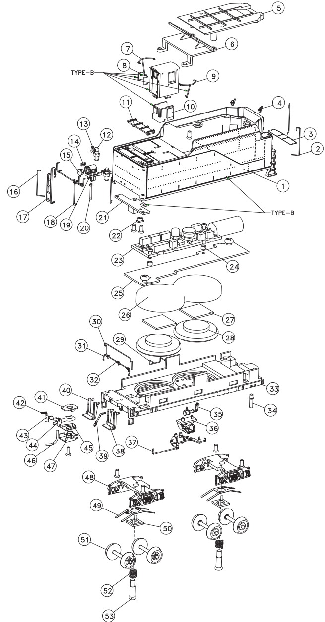
PRR L1s Tender - Late Type w/ Brakeman's Cab
