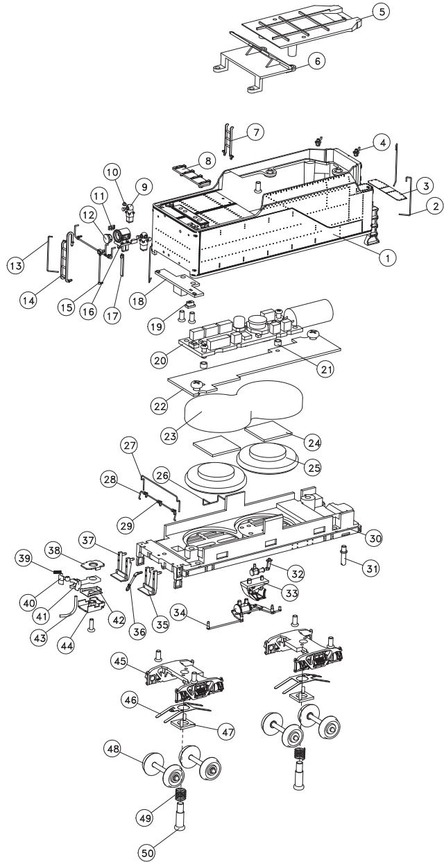
PRR L1s Tender Early Type
