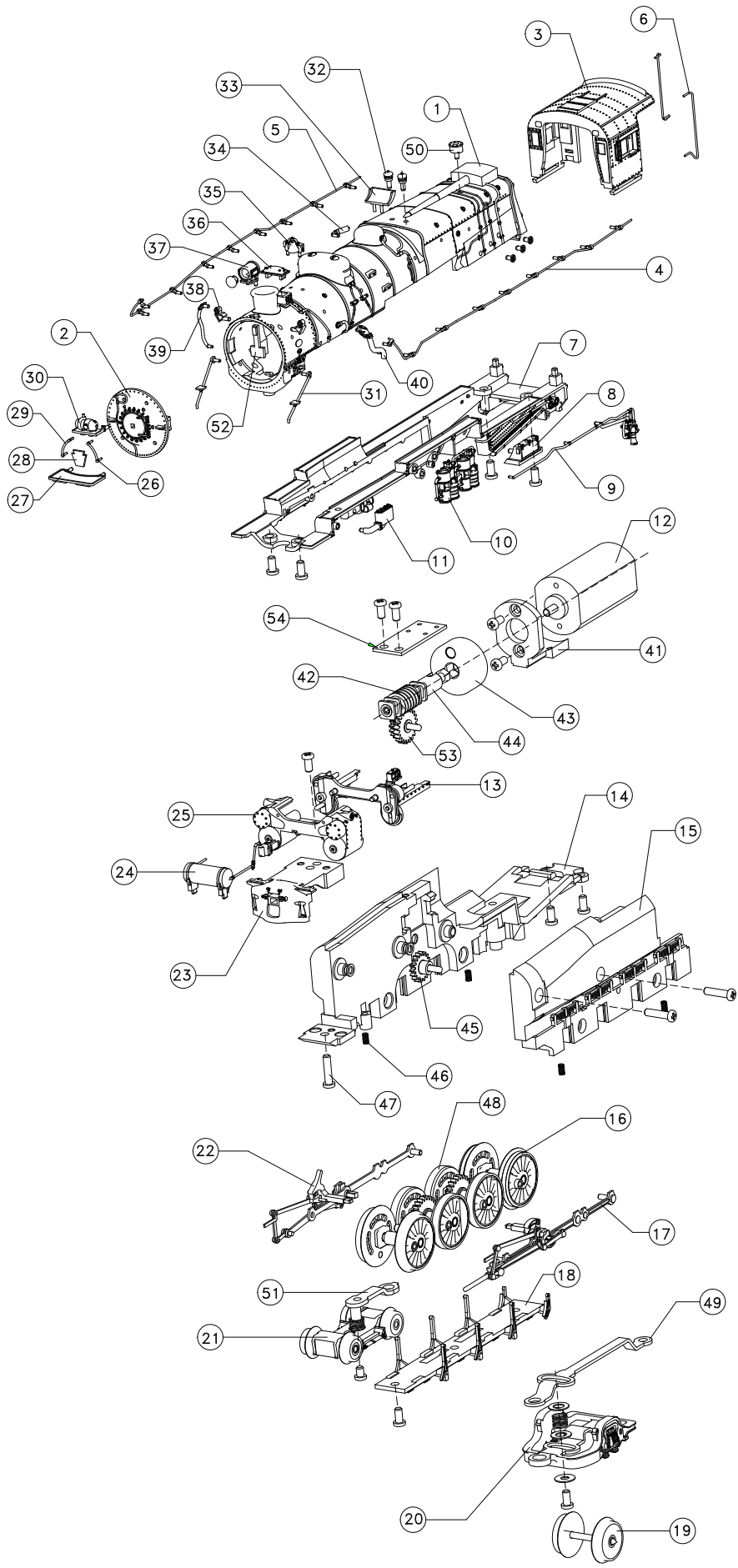
PRR M1b 4-8-2, N Scale Exploded View Diagram
