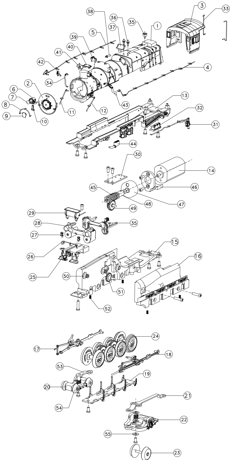
PRR M1a 4-8-2, N Scale Exploded View Diagram
