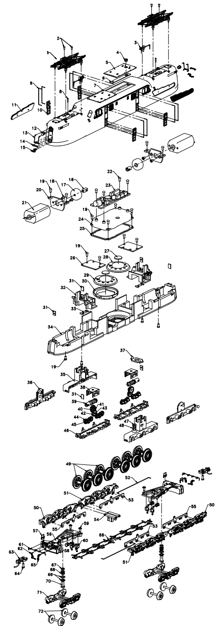
GG1-5STRIP-FIXED-COUPLER
