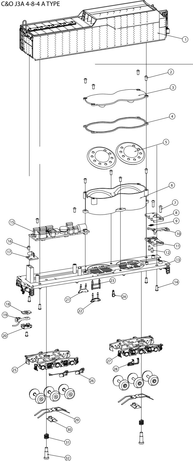
C&O J3A 4-8-4 A TYPE
