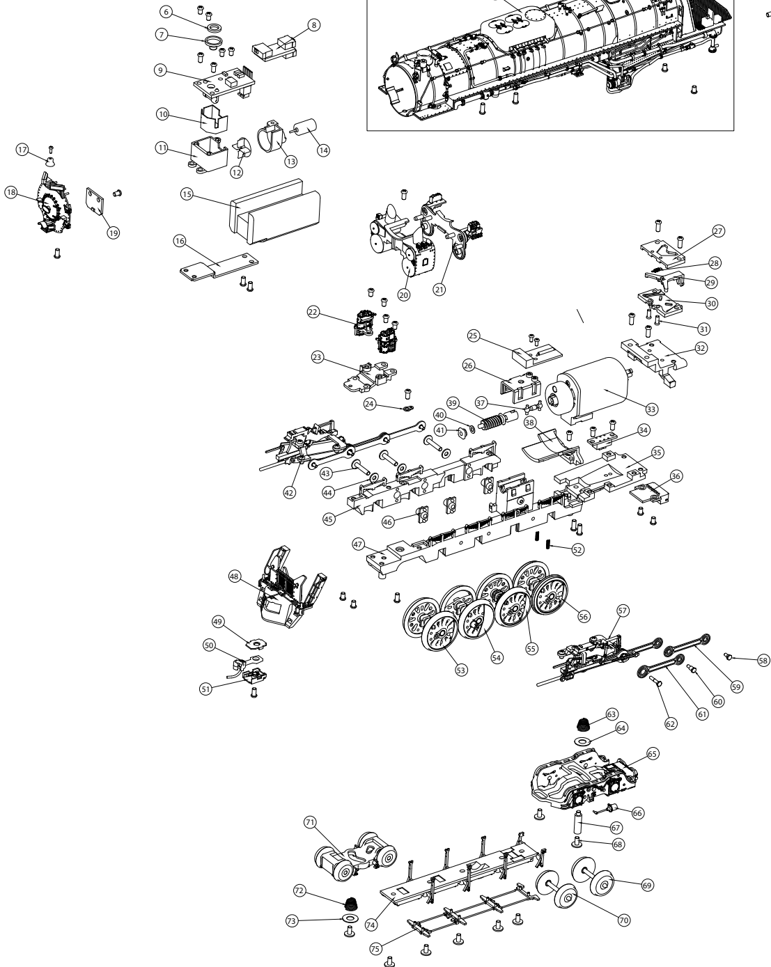
C&O J3A 4-8-4 A TYPE
